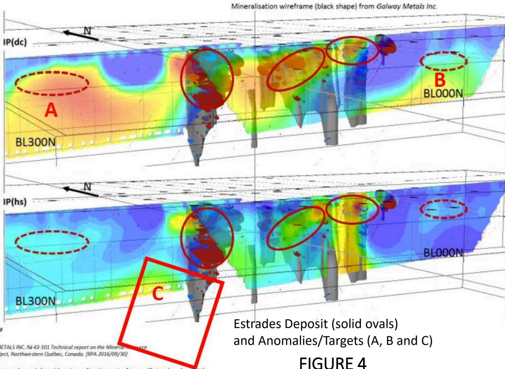
Figure 4-2: BL300N + BLO00N: view in 3D of the IP(dc; top) and IP(hs; bottom) models with mineralisation wireframe (Estrades deposit).
