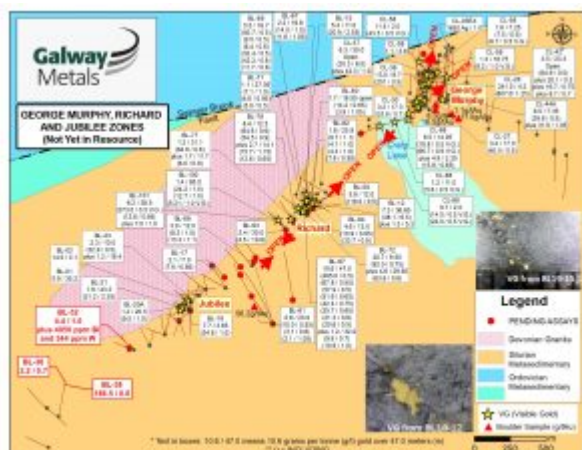
Figure 2: Strong Gold-in Glacial Till, Soil, Boulders and Chip Samples at Clarence Stream
